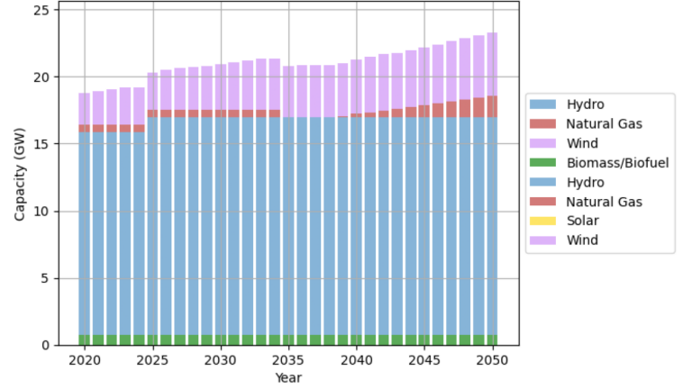
Yearly Total Capacity for Different Technologies - REF Case
