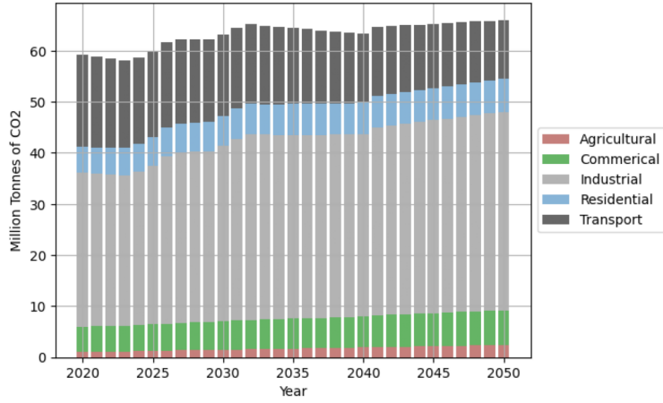
Yearly Emission by Sector - REF Case
