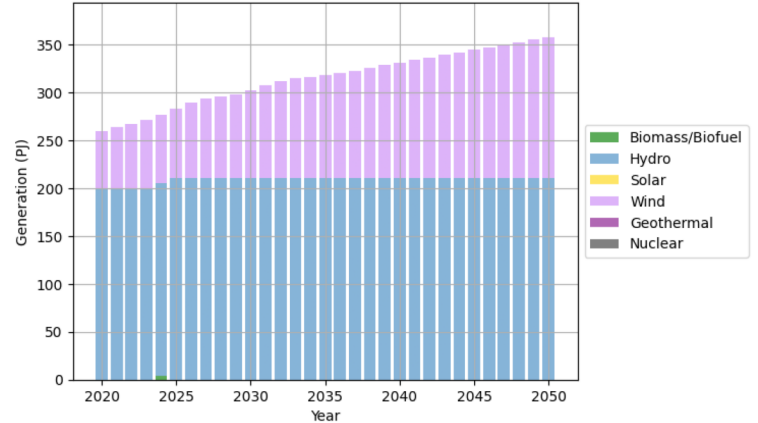
Yearly Generation for Different Technologies - REF Case
